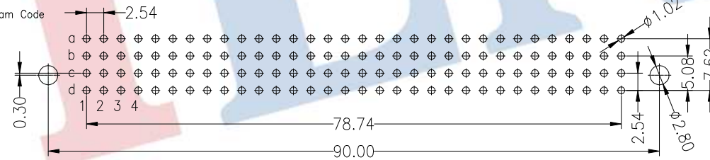
Recommended P.C.B Layout(Top Side) (PCB BOARD TOLERANCE±0.05)
