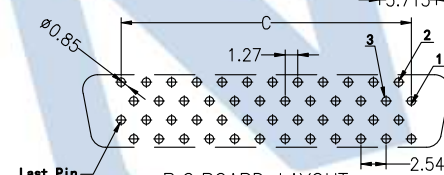
P.C. BOARD LAYOUT (68,100Pin) R1 Type / 正脚位
