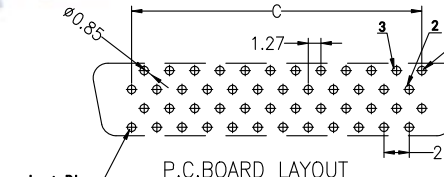
P.C. BOARD LAYOUT (68,100Pin) R2 Type / 反脚位
